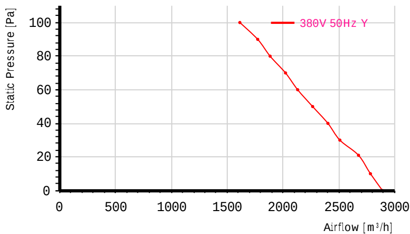
Airflow curve
