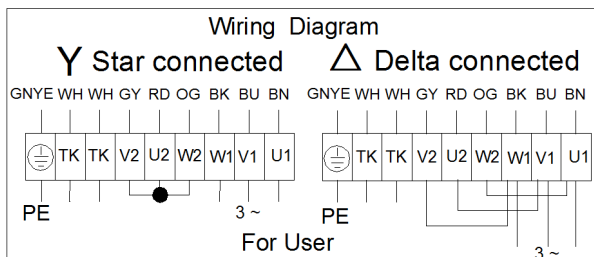
Wiring diagram (Default without thermal protector)
