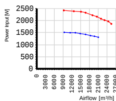
Power input
