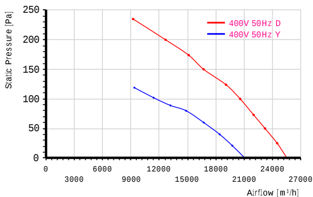
Performance curve
